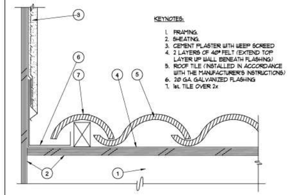
TILE @ WALL DETAIL
