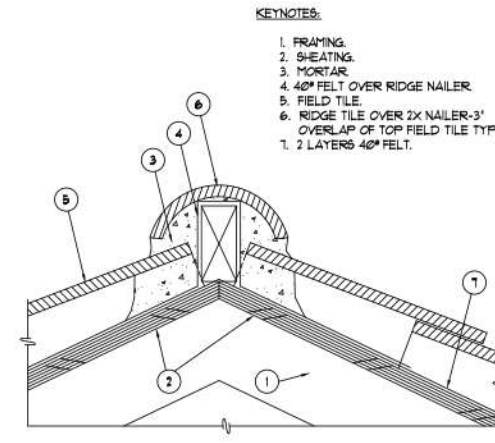
TILE @ RIDGE OR OR HIP DETAIL
