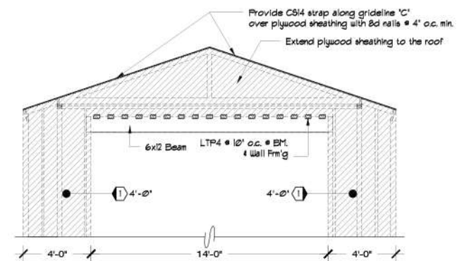
Shear transfer @ garage door opening
