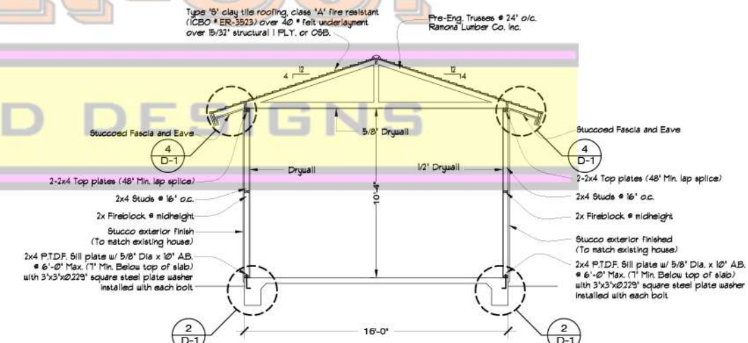
SECTION B
