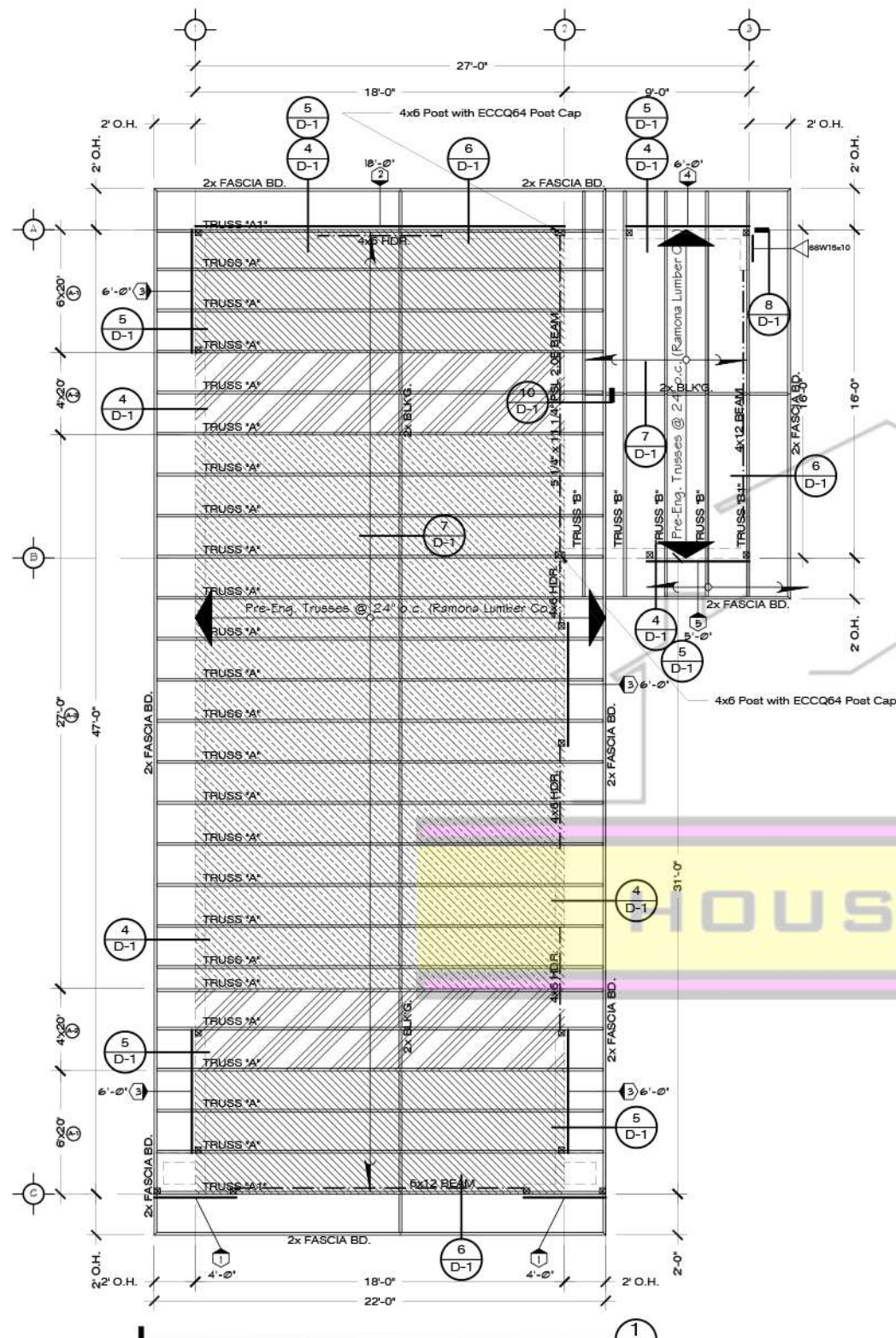
GARAGE ROOF FRAMING PLAN
