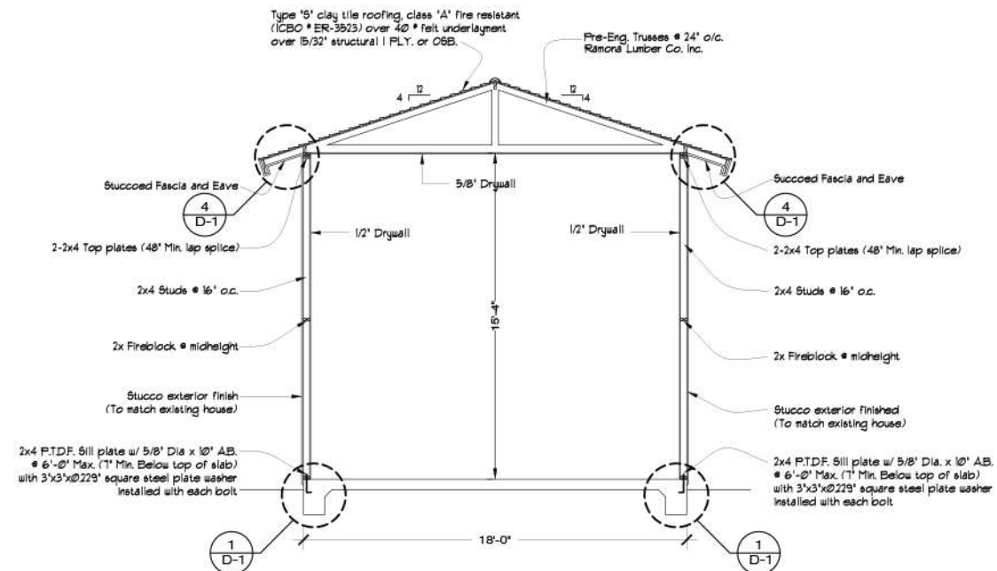
SECTION A
