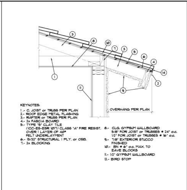
ENHANCED EAVE DETAIL
