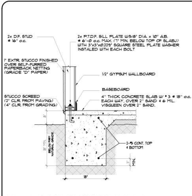
FOOTING DETAIL-1 (18'x18')
