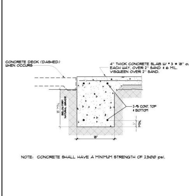
FOOTING AT GARAGE DOOR
