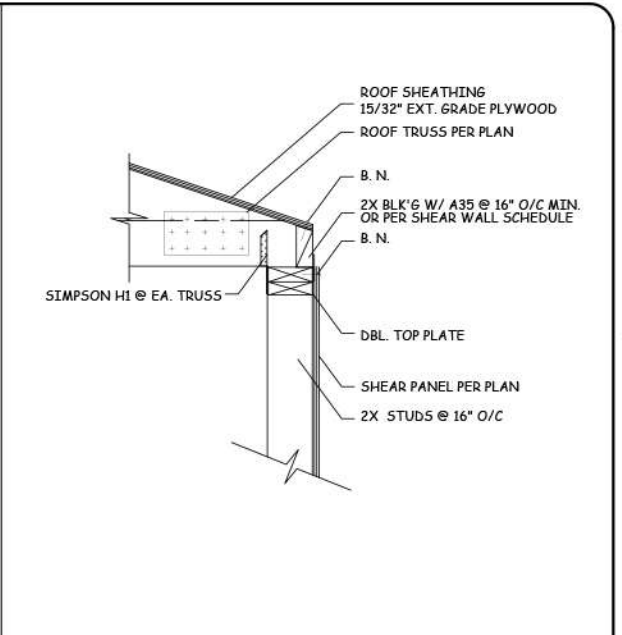
SHEAR TRANSFER AT EAVE DETAIL
