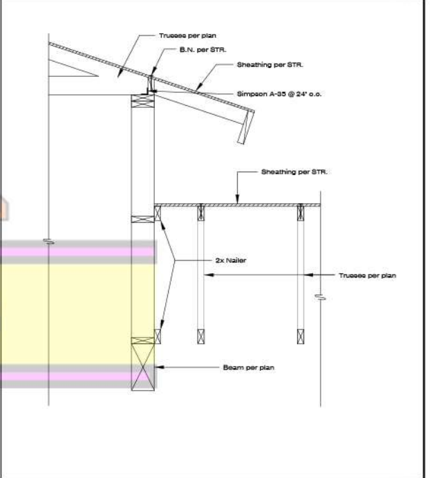
BEAM & ROOFS DETAIL
