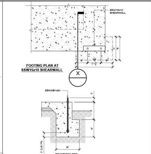
STEEL STRONG-WALL FOUNDATION DETAIL
