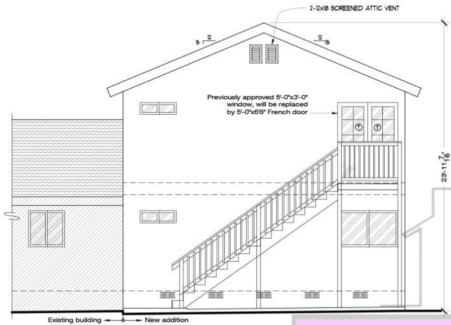
EAST (REAR) ELEVATION
