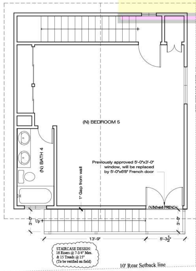
(N) UPPER FLOOR PLAN
