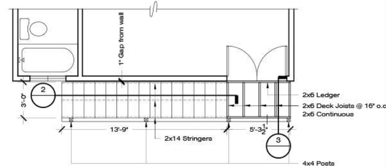
STAIR FRAMING PLAN
